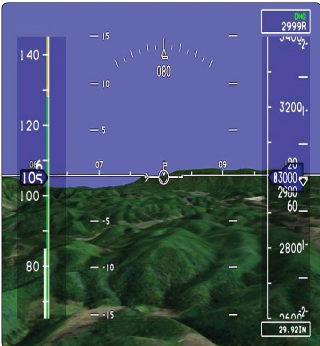
Figure 17-24. SVS system.
