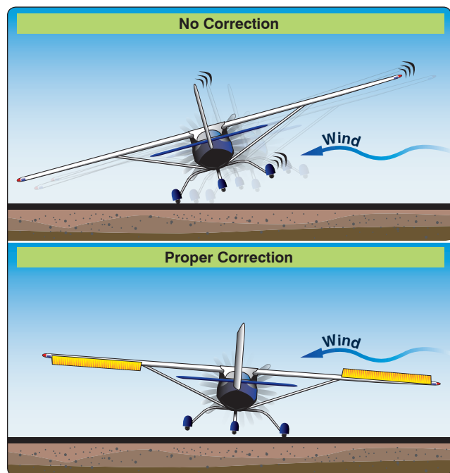
Figure 5-5. Crosswind effect.
