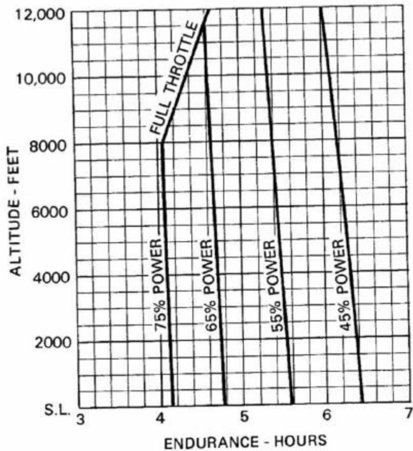
Figure 5-9. Endurance Profile (Sheet 1 of 2)
